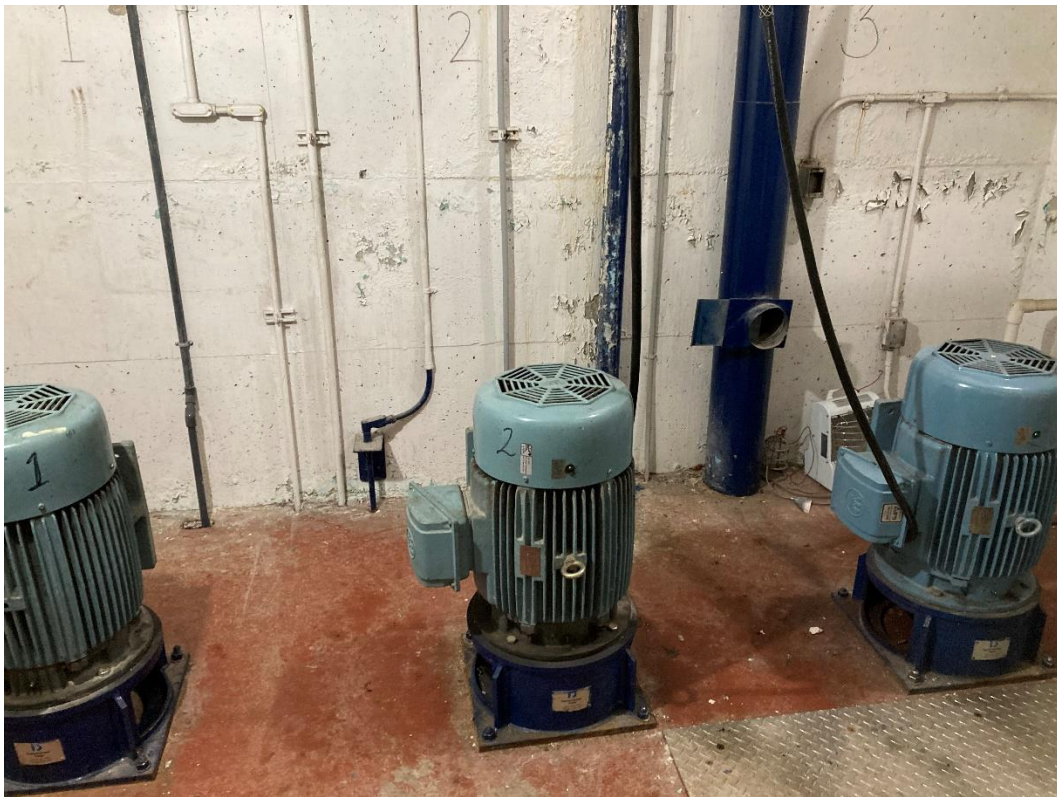
Motor Room – Lift Pump Motors, 30 HP each
