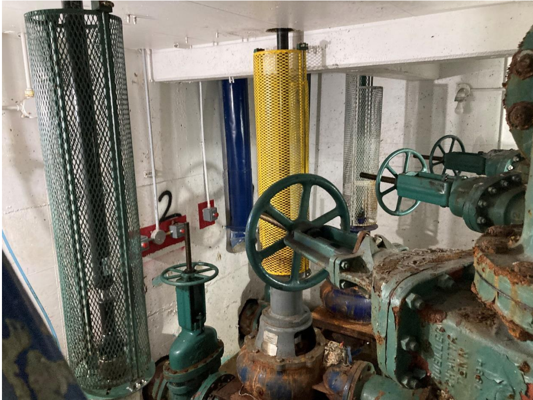
Pump Room – lift pumps and piping
